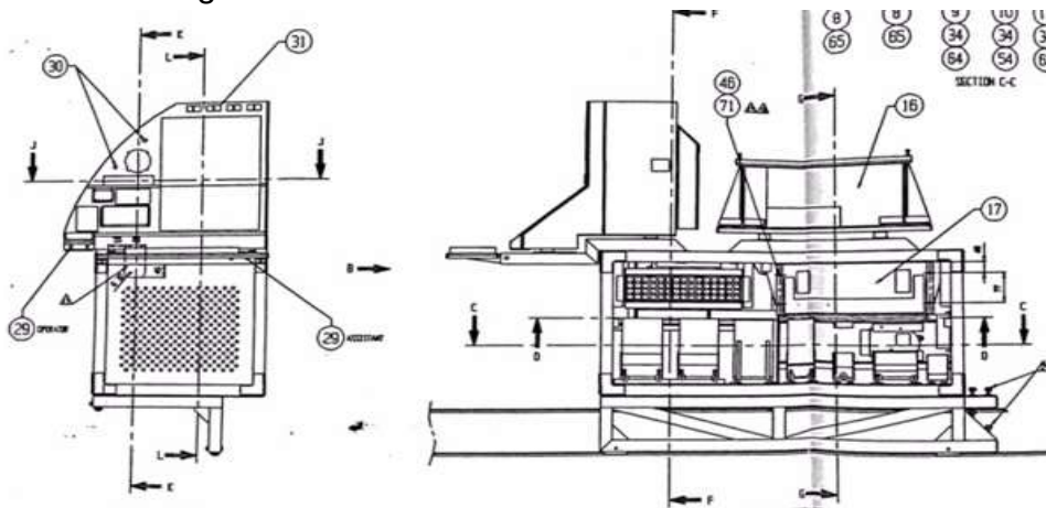
Fig 20.1 FIS Drawing
