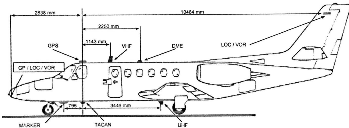
Fig 20.4 FIS Antenna Positioning Side View
