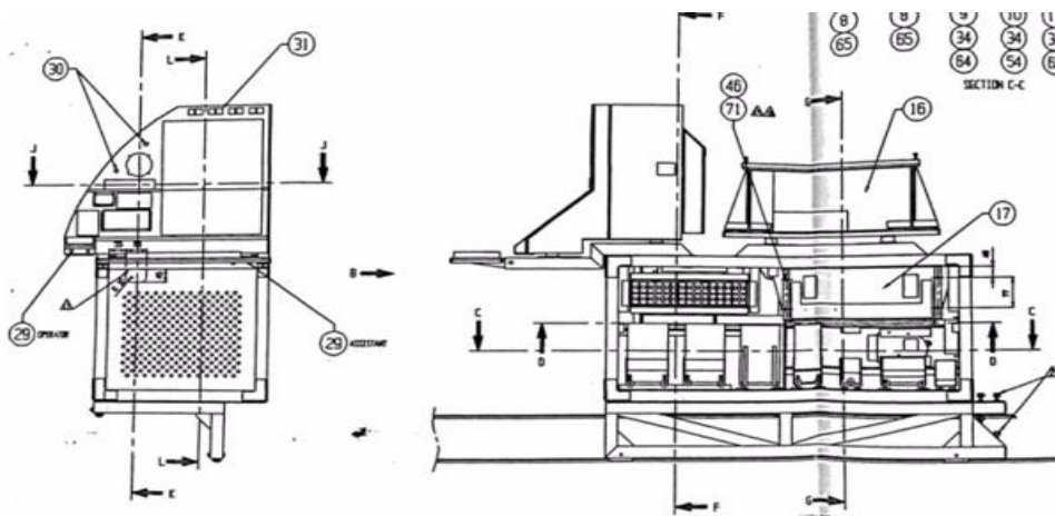
Fig 20.1 FIS Drawing
