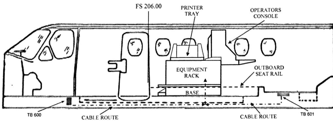
Fig 20.2 FIS Positioning Side View
